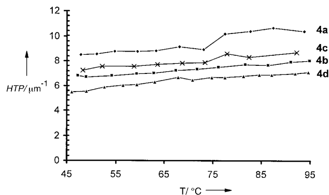
Figure 3. Helical twisting power of the investigated optically active compounds 4a–d versus temperature. The compounds induce the formation of left-handed helices.
